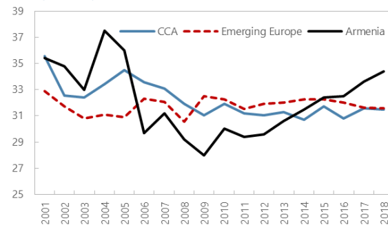
Gini Index (2001-18)
