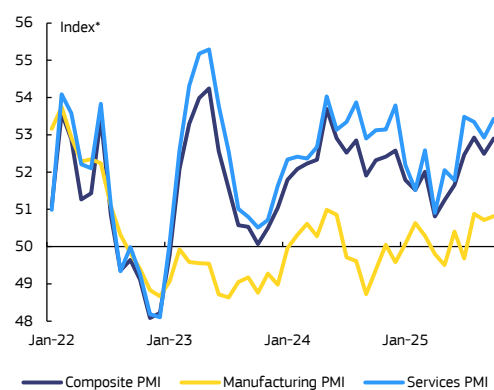
Graph I.2.2: Global PMIs
